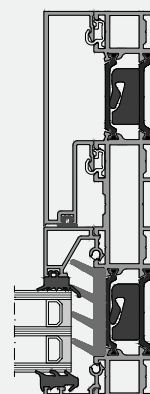
Fixed glazing (FO, GO)
