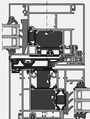
Central Mullion
